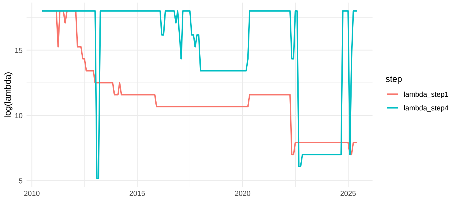
TVP-Factor, h=12: Step1 vs Step4 lambdas (log)
