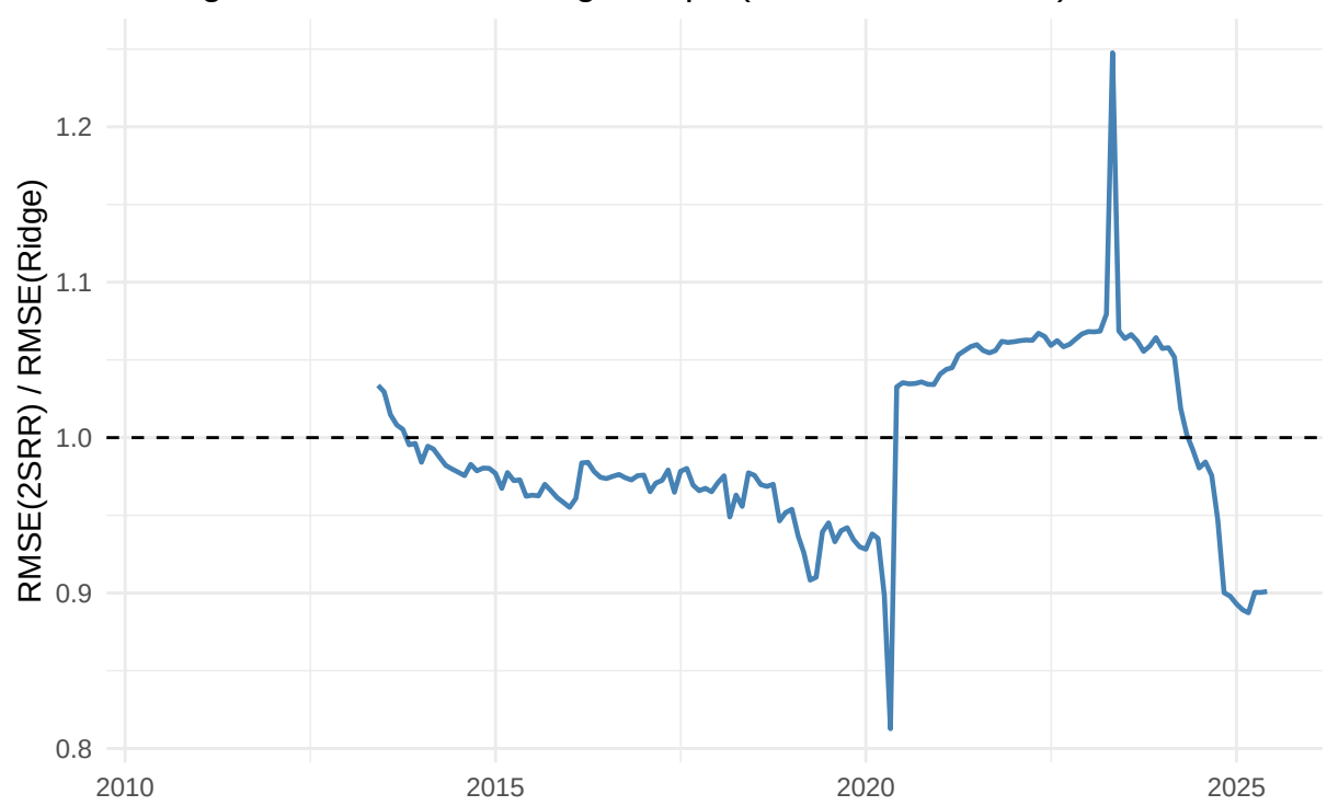
Rolling RMSE Factor vs Ridge Step1 (36-month window), h=12
