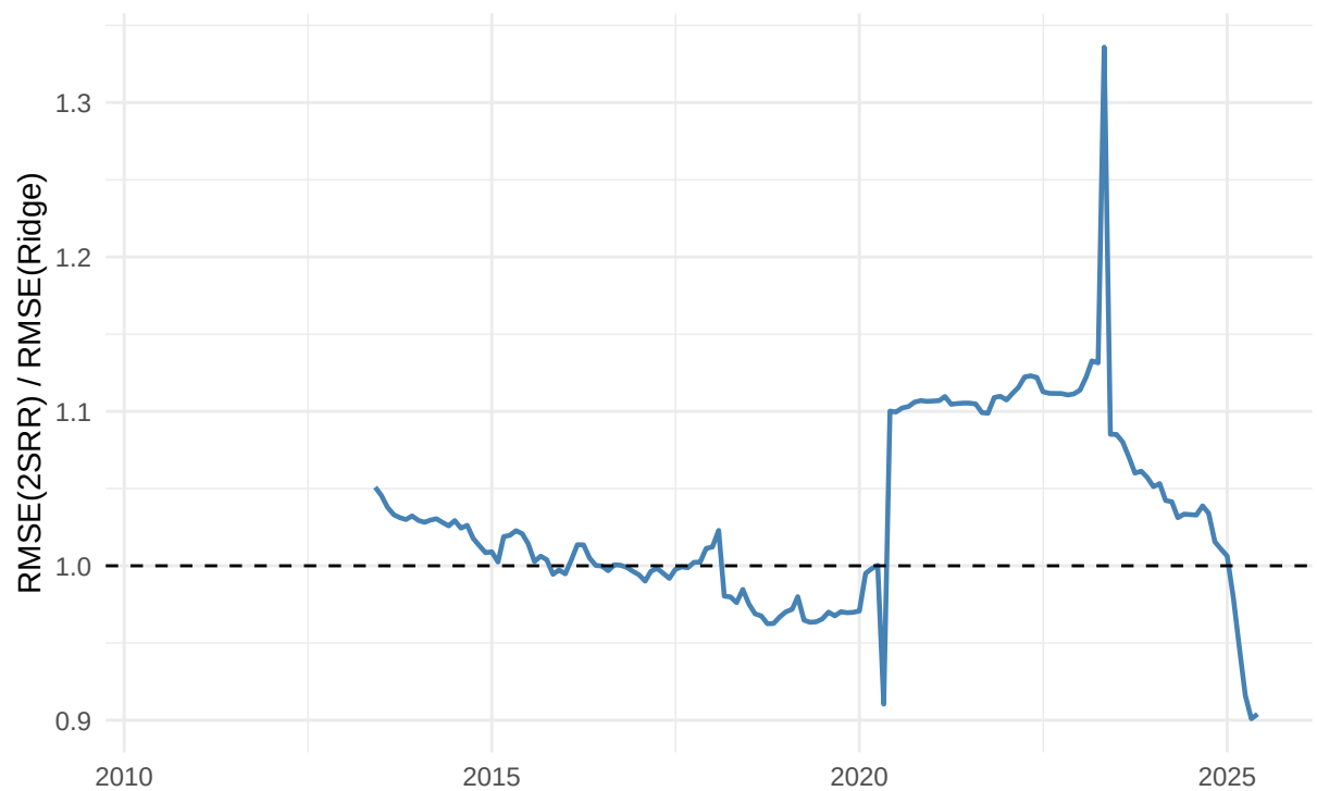
Rolling RMSE Factor vs Ridge Step1 (36-month window), h=3
