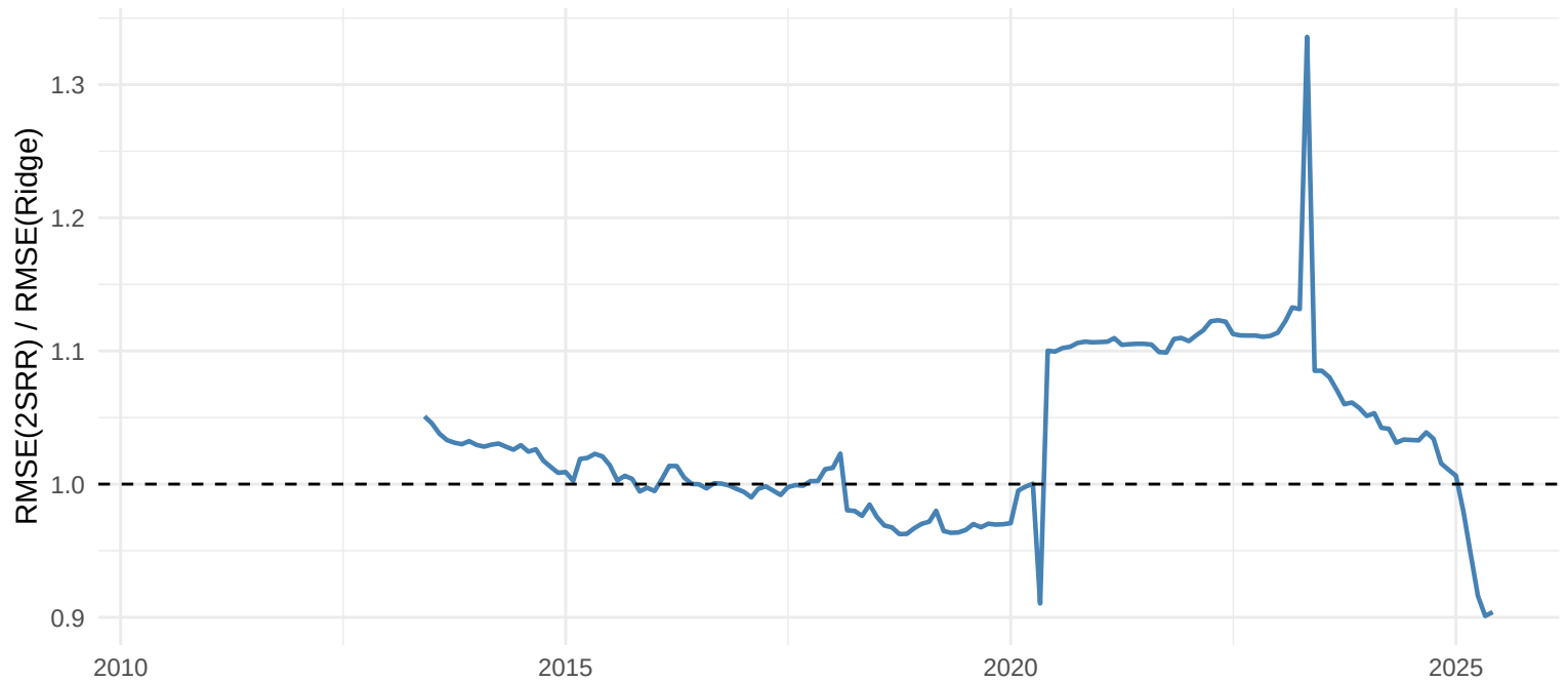
Rolling RMSE Factor vs Ridge Step1 (36-month window), h=3
