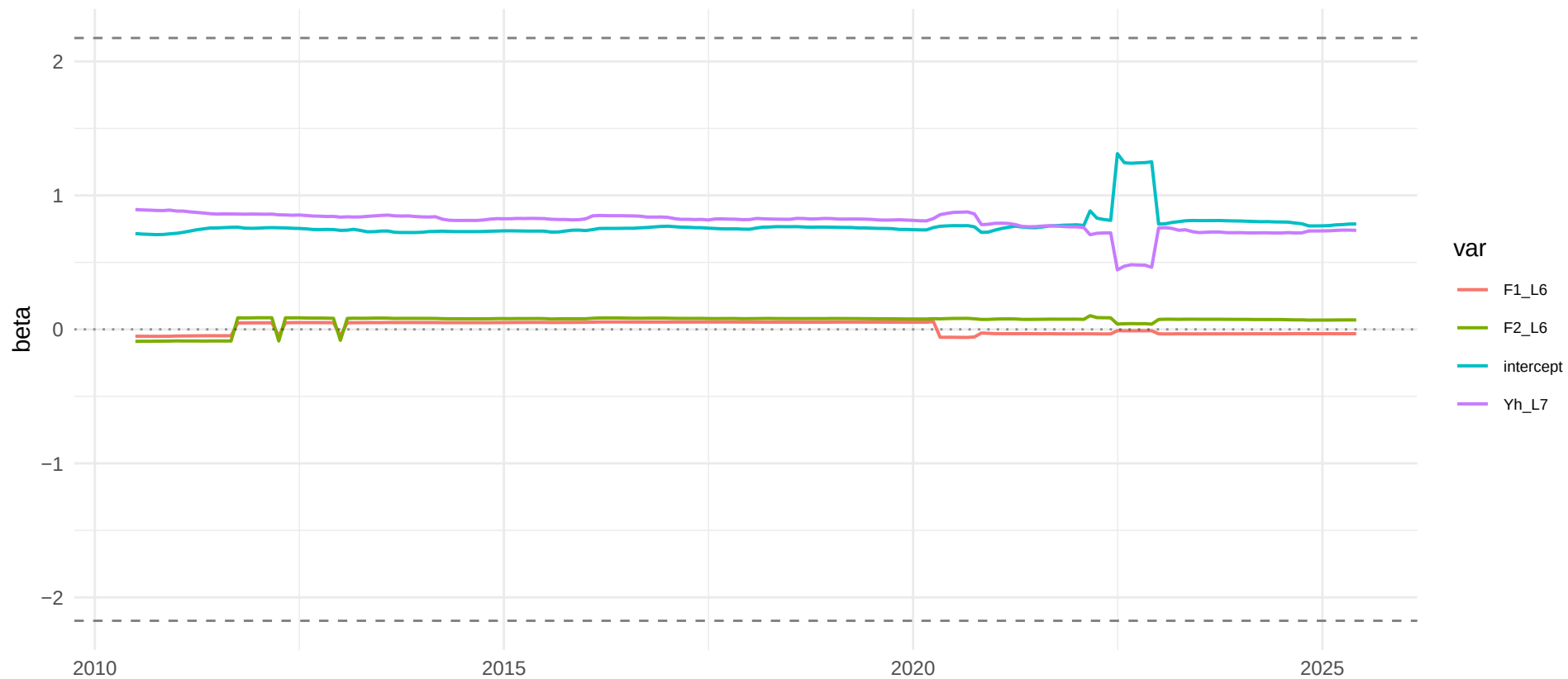
h=6: top-4 betas TVP (FAVAR) vs Ridge constante ( |\text{beta}|=2.174 )
