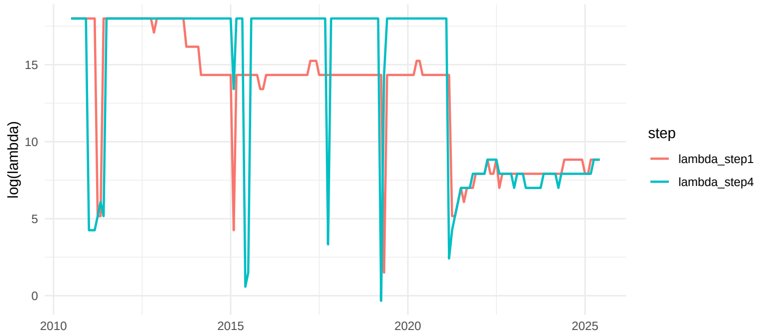
TVP-AR, h=1 : lambdas Step1 vs Step4 (log)
