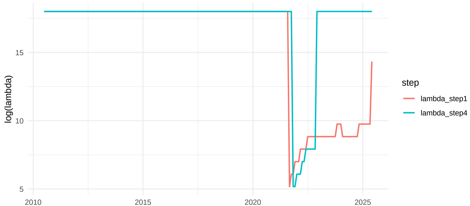
TVP-AR, h=6: lambdas Step1 vs Step4 (log)
