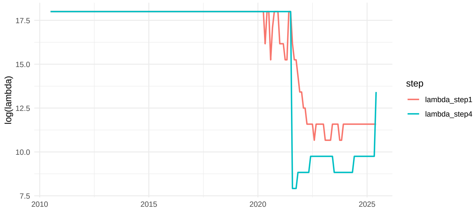
TVP-FAVAR, h=3: lambdas Step1 vs Step4 (log)
