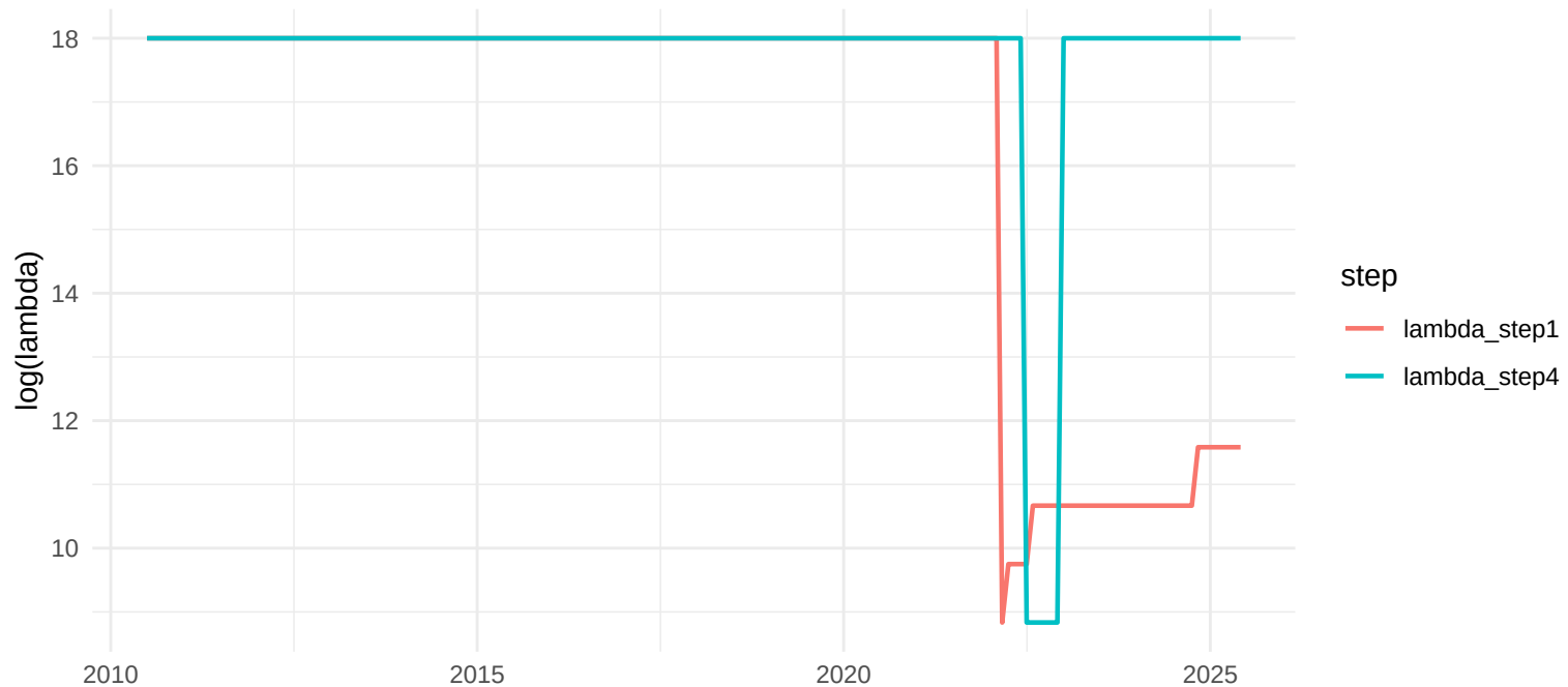
TVP-FAVAR, h=6: lambdas Step1 vs Step4 (log)
