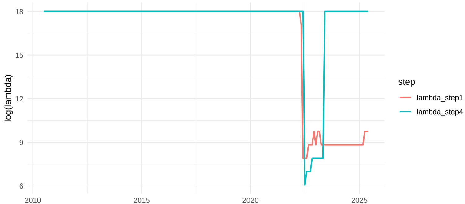
TVP-FAVAR, h=12: lambdas Step1 vs Step4 (log)
