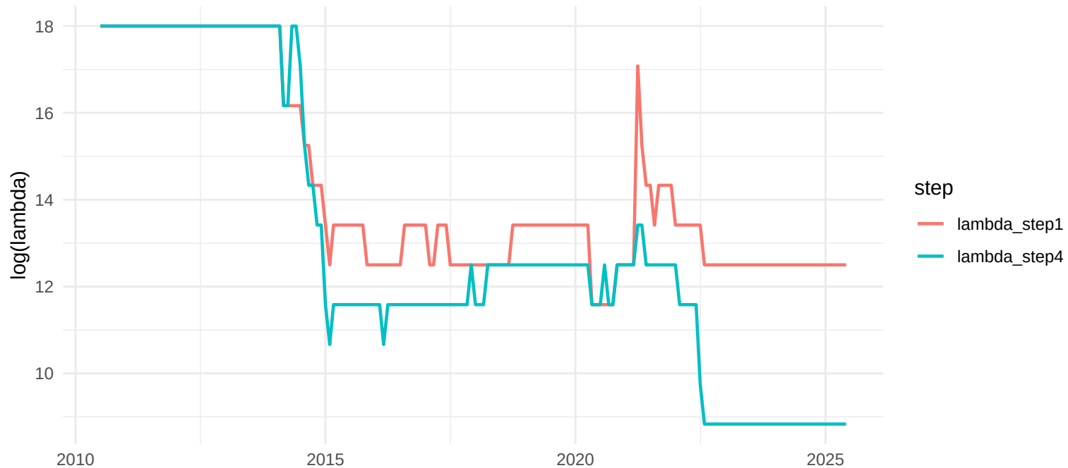
TVP-Factor, h=1: lambdas Step1 vs Step4 (log)
