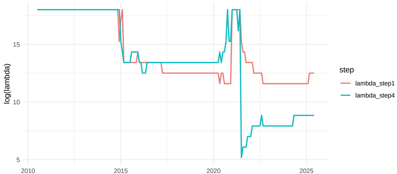
TVP-Factor, h=3: lambdas Step1 vs Step4 (log)
