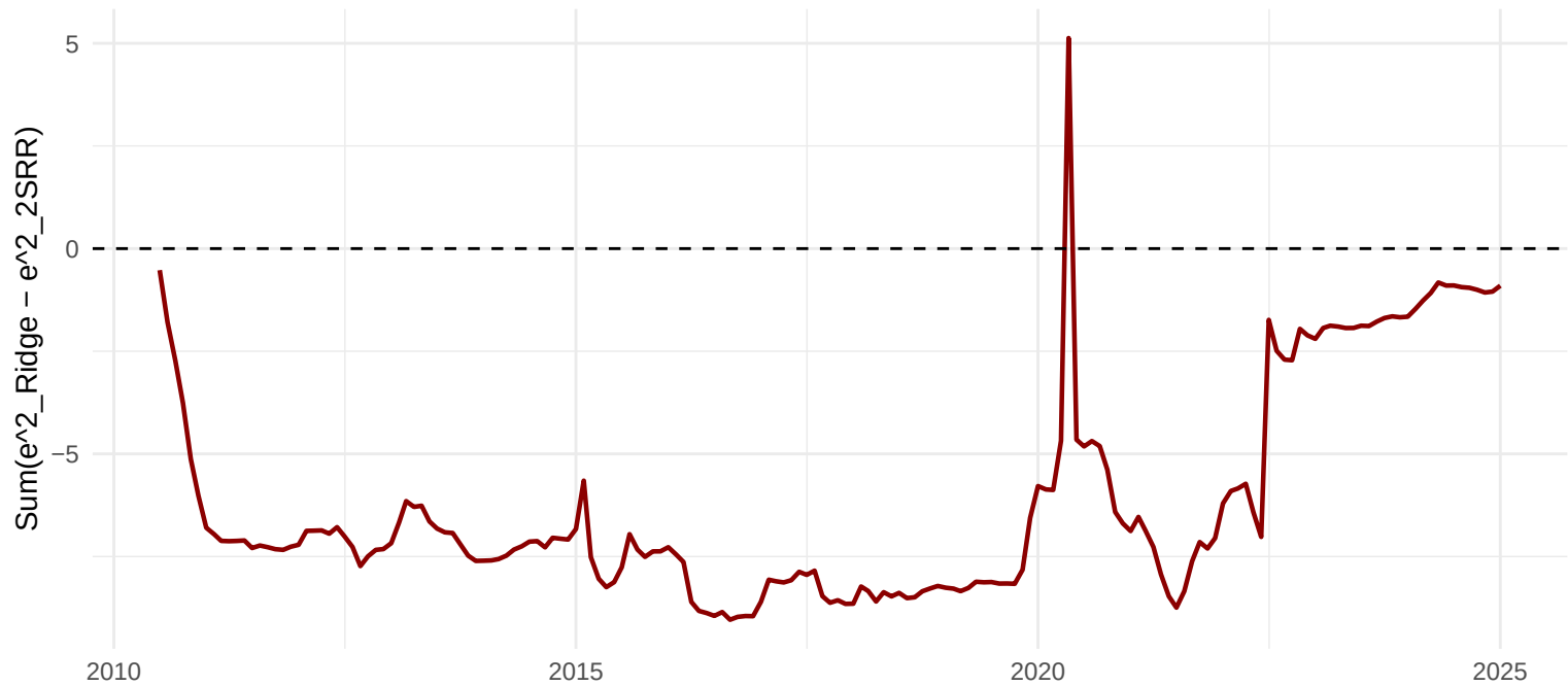
CSSED 2SRR-FAVAR vs Ridge Step1, h=6
