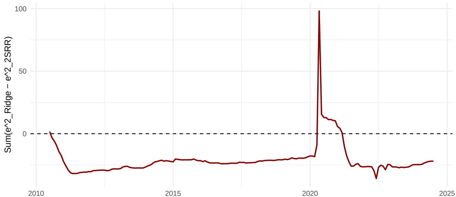
CSSED 2SRR-FAVAR vs Ridge Step1, h=12
