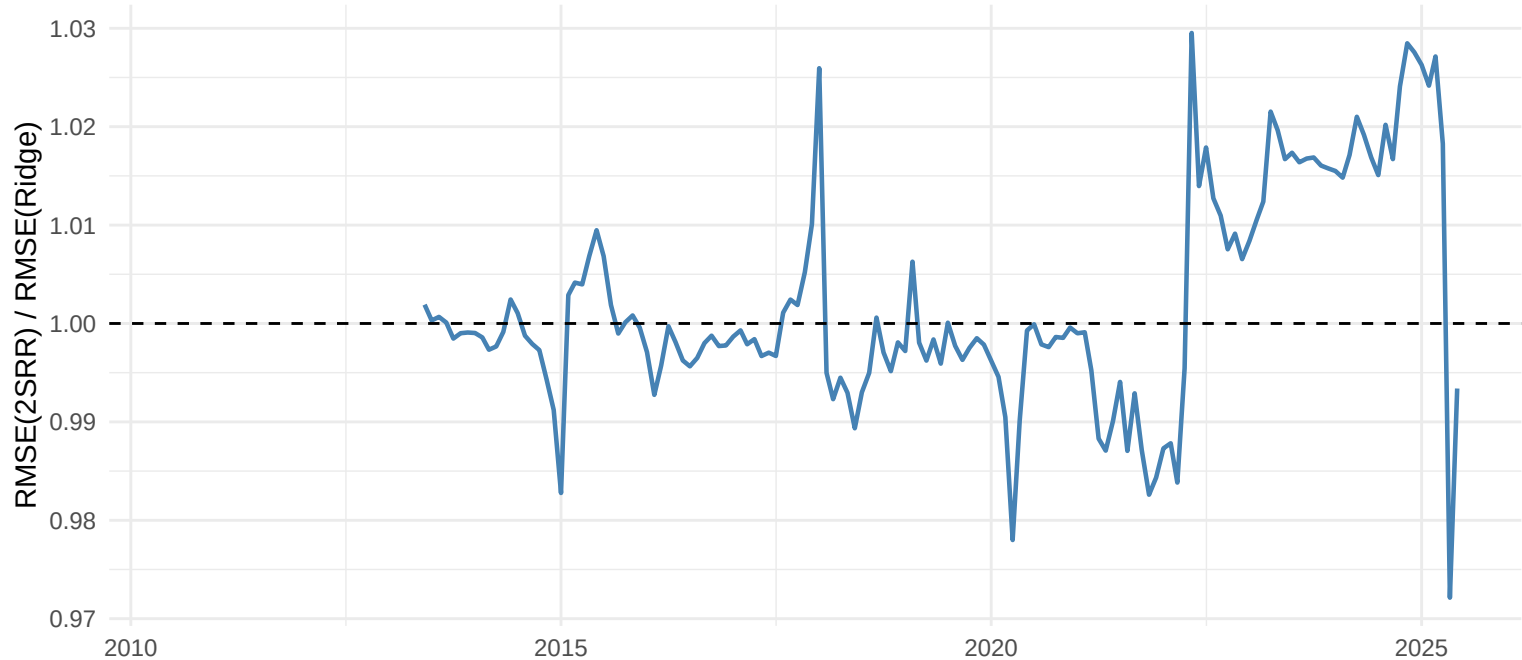
Rolling RMSE AR vs Ridge Step1 (janela 36), h=1
