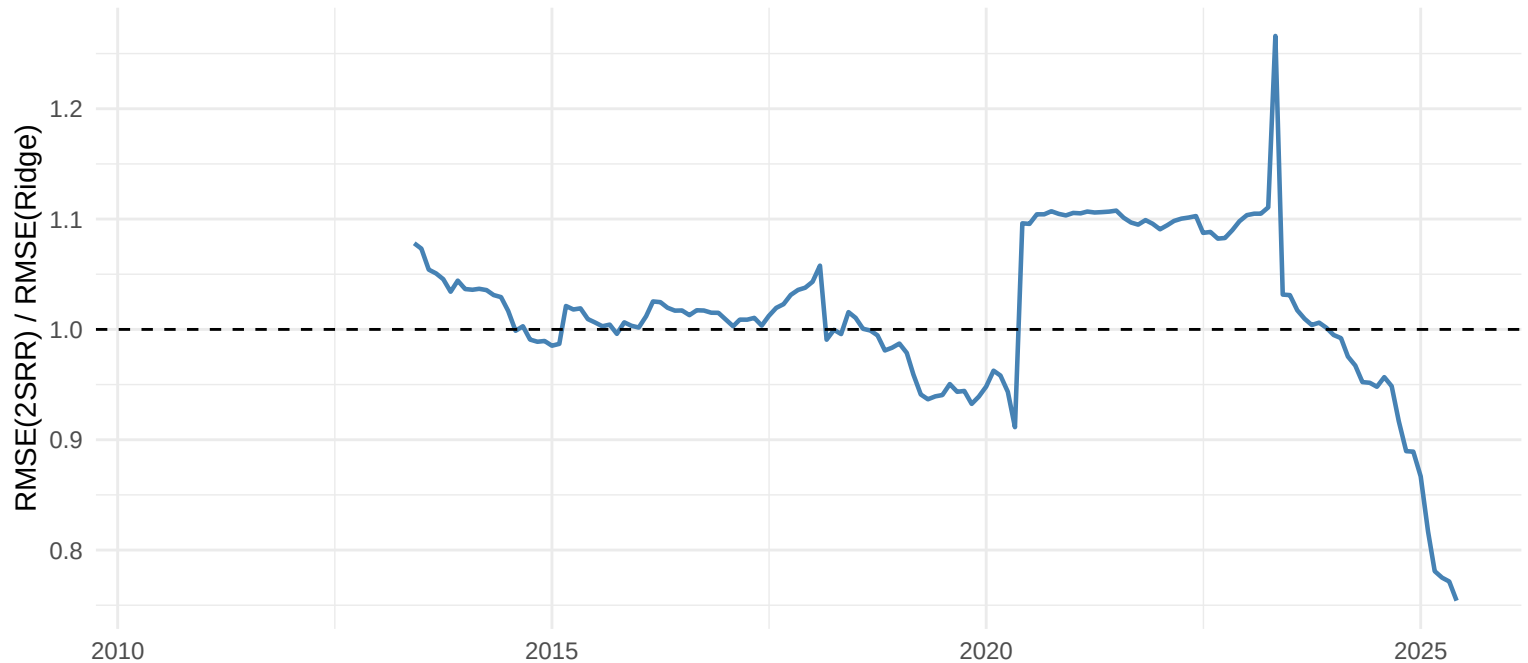
Rolling RMSE Factor vs Ridge Step1 (janela 36), h=6
