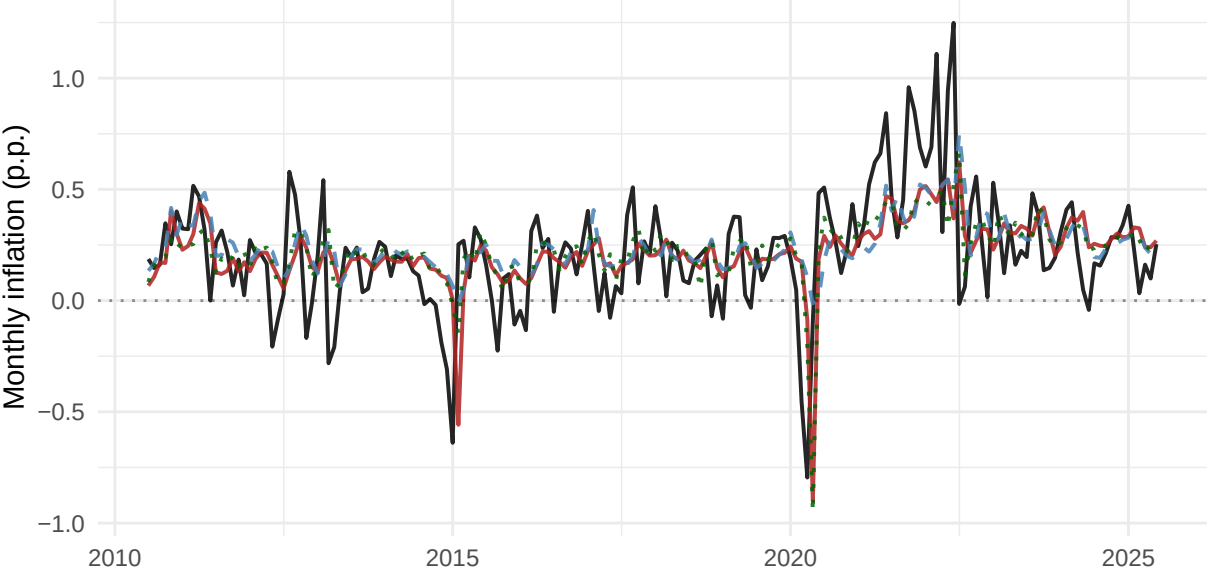
2SRR (3 cases) vs monthly realized, h=3
