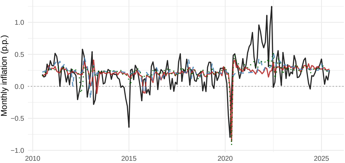
2SRR (3 cases) vs monthly realized, h=12
