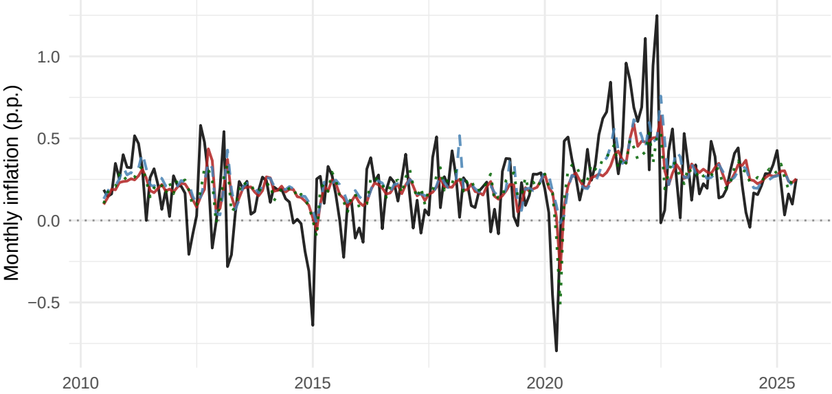
2SRR (3 cases) vs monthly realized, h=6
