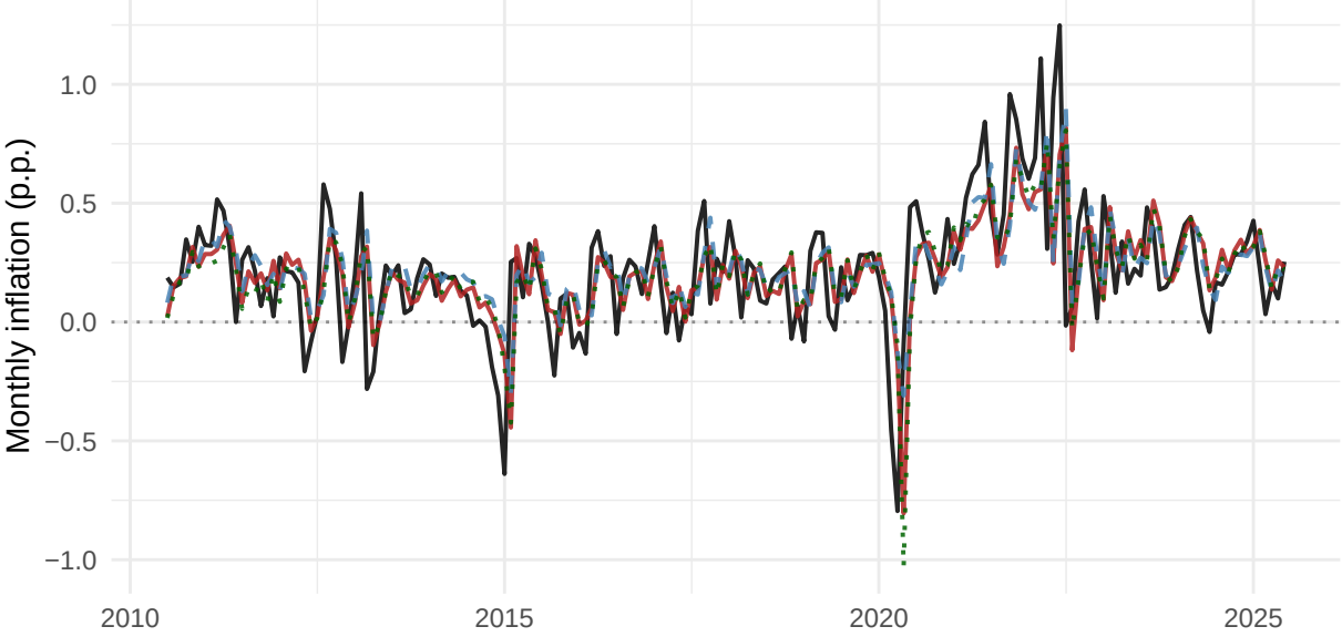
2SRR (3 cases) vs monthly realized, h=1
