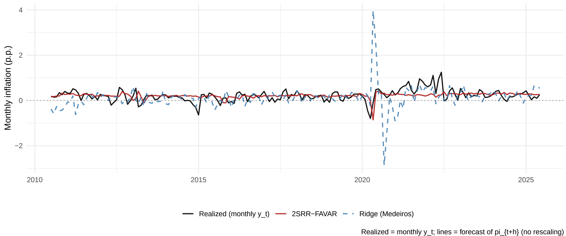
2SRR-FAVAR vs classical Ridge (Medeiros), h=12
