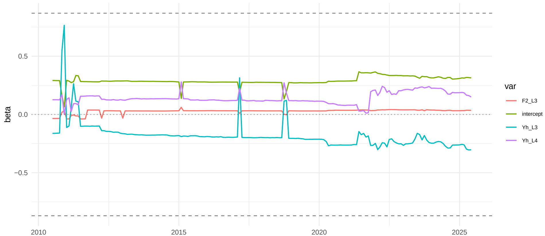
h=3: top-4 TVP (FAVAR) betas vs constant Ridge ( |\text{beta}|=0.869 )
