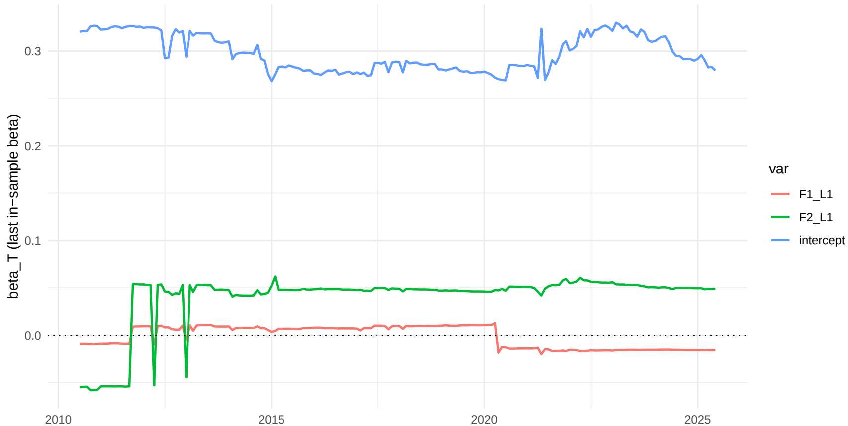
TVP-Factor, h=1: top-3 betas (by sd)
