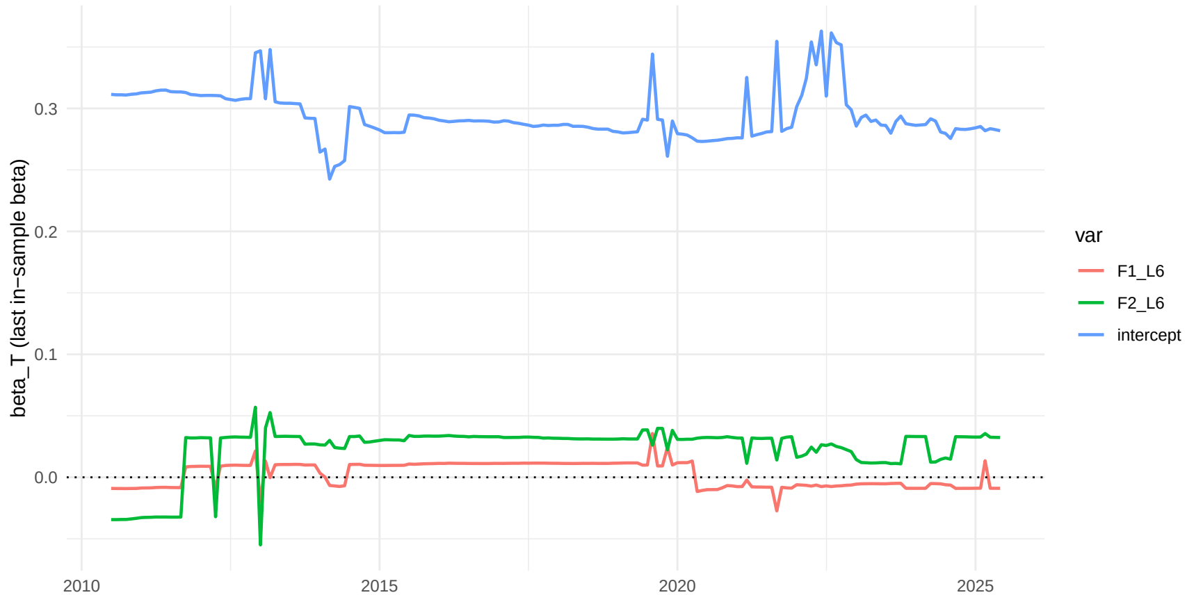
TVP-Factor, h=6: top-3 betas (by sd)
