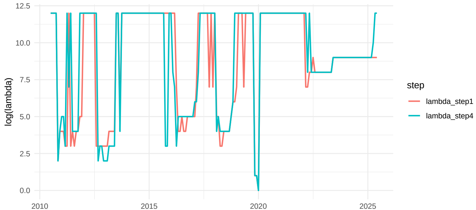
TVP-FAVAR, h=12: Step1 vs Step4 lambdas (log)
