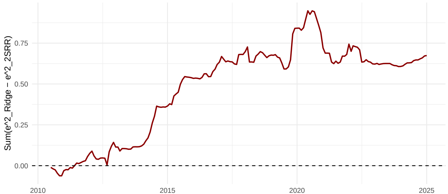
CSSSED 2SRR-AR vs Ridge Step1, h=6
