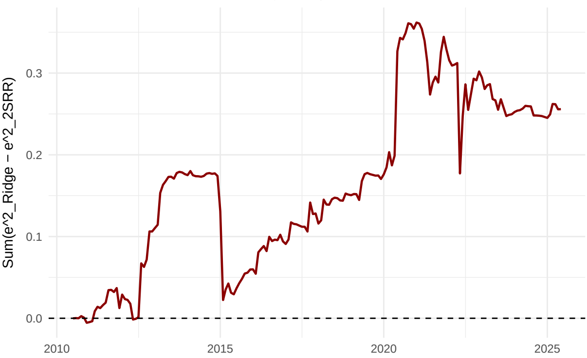
CSSSED 2SRR-FAVAR vs Ridge Step1, h=1
