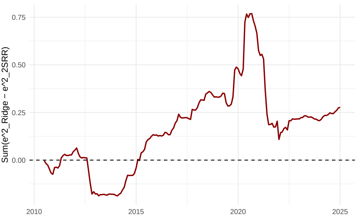
CSSSED 2SRR-FAVAR vs Ridge Step1, h=6
