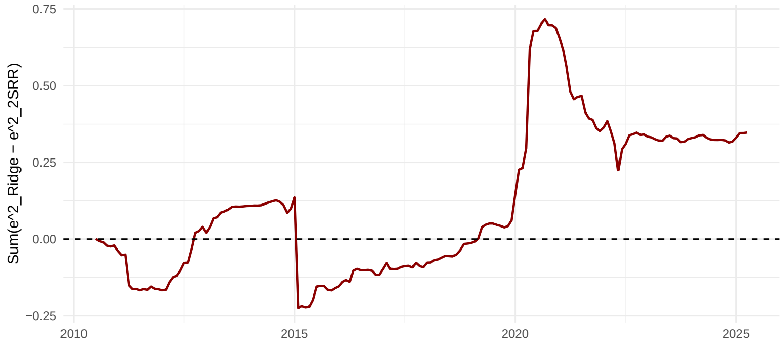
CSSED 2SRR-FAVAR vs Ridge Step1, h=3
