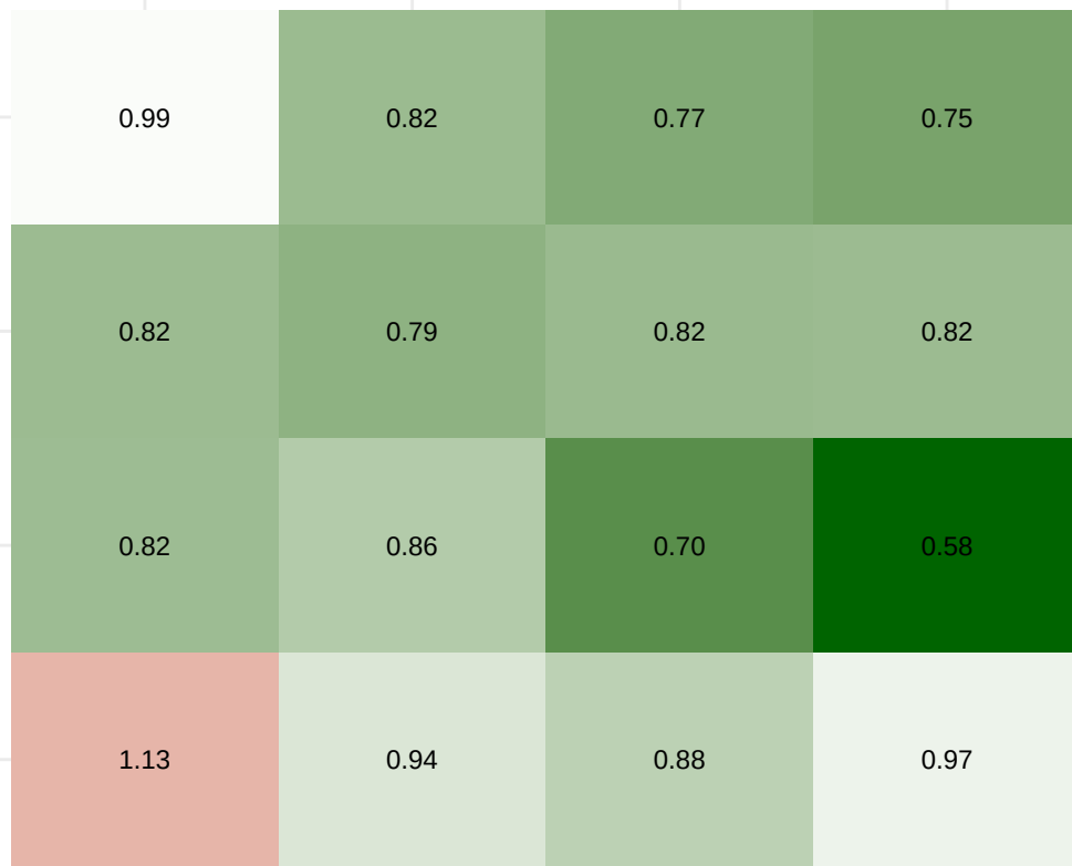
TVP-FAVAR: RMSE relative to RW per sub-period
