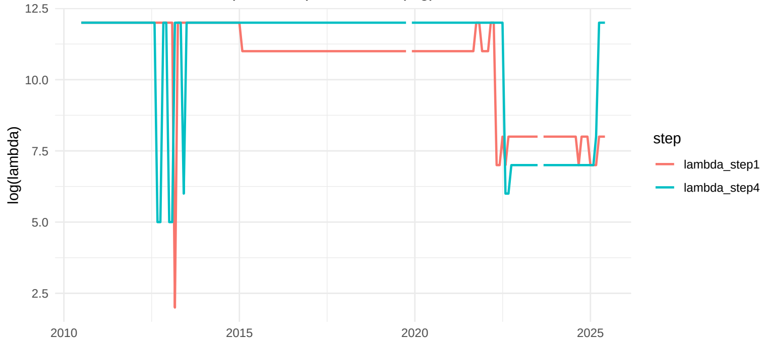
TVP-Factor, h=12: Step1 vs Step4 lambdas (log)
