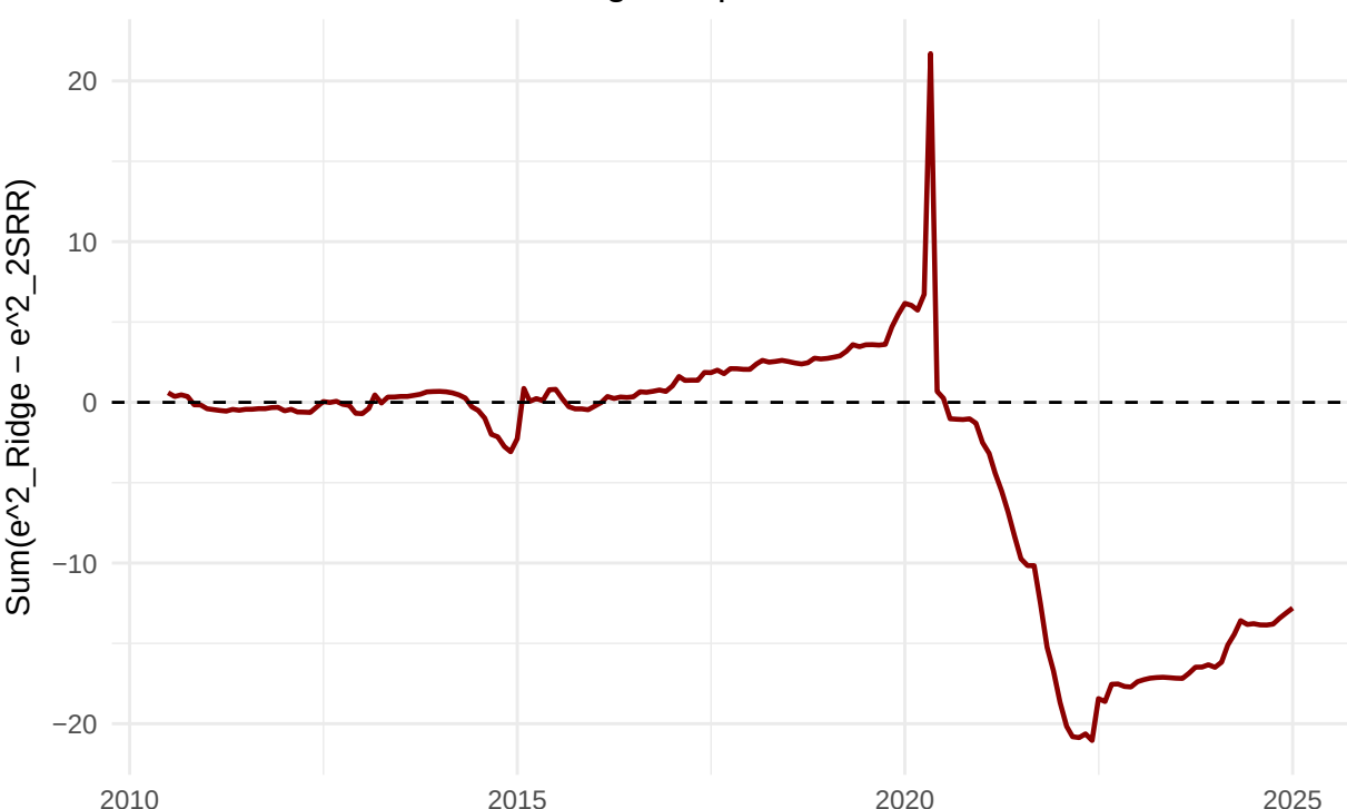
CSSSED 2SRR-Factor vs Ridge Step1, h=6
