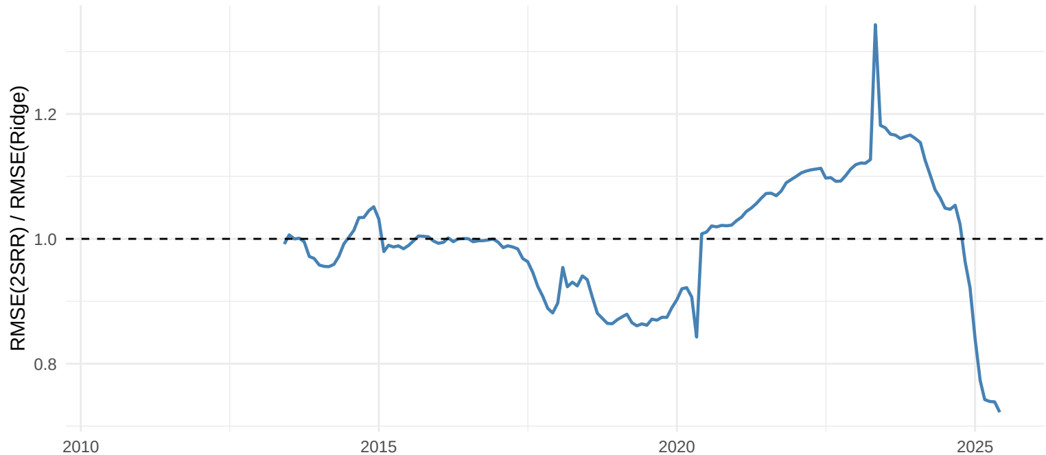
Rolling RMSE Factor vs Ridge Step1 (36-month window), h=6
