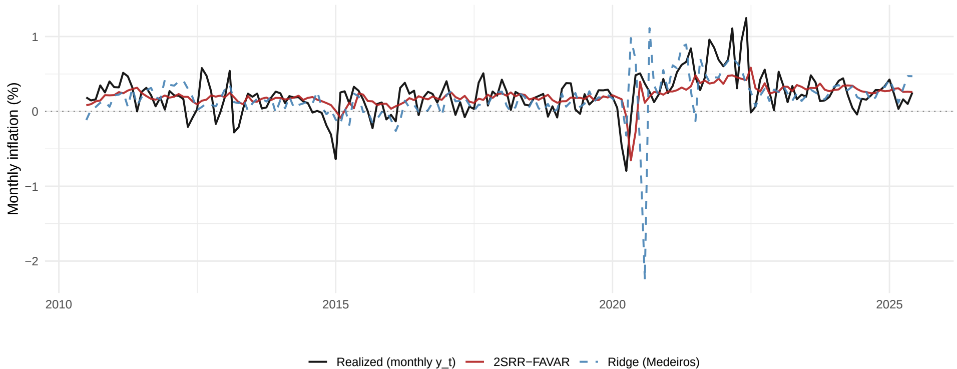
2SRR-FAVAR vs classical Ridge (Medeiros), h=3
