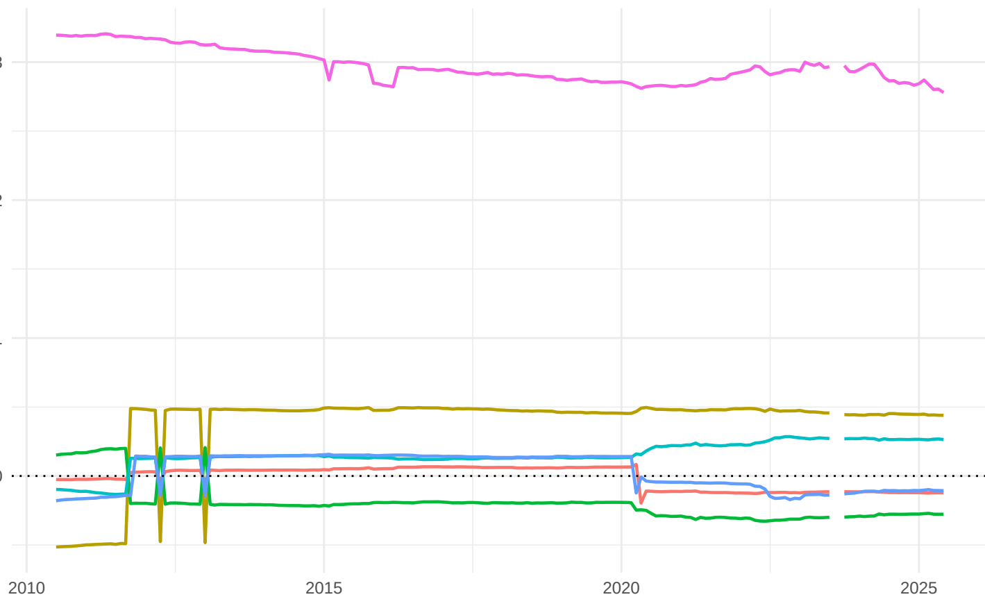
TVP-Factor, h=1: top-6 betas (by sd)
