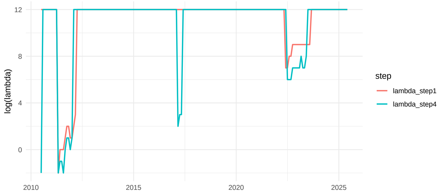
TVP-AR, h=12: Step1 vs Step4 lambdas (log)
