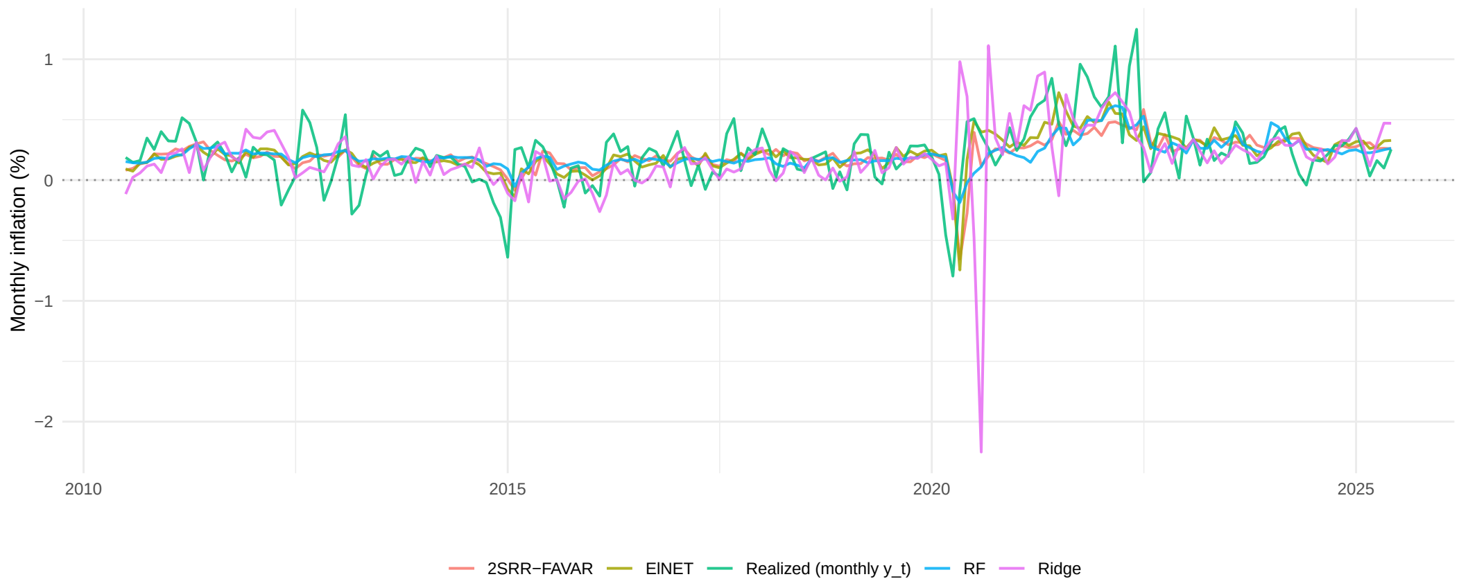
Forecasts h=3 (monthly scale): 2SRR-FAVAR + 2 best + worst Medeiros
