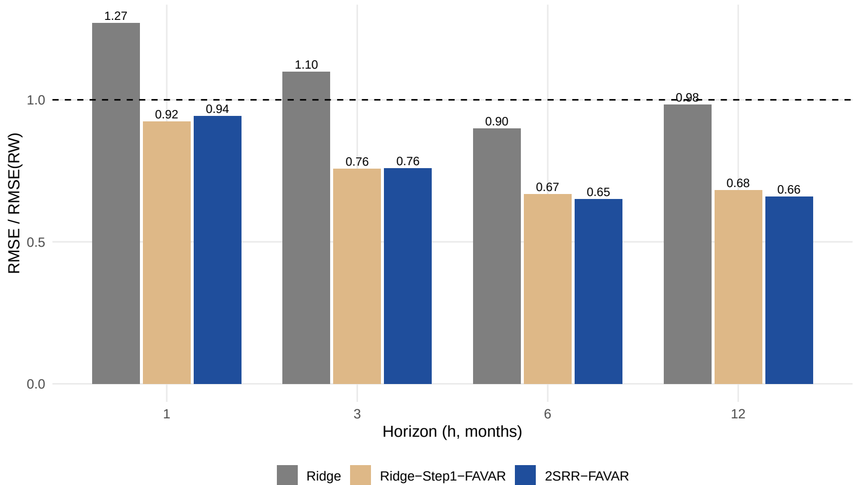
2SRR-FAVAR against the ordinary 117-series ridge and its own static (Step-1) counterpart
