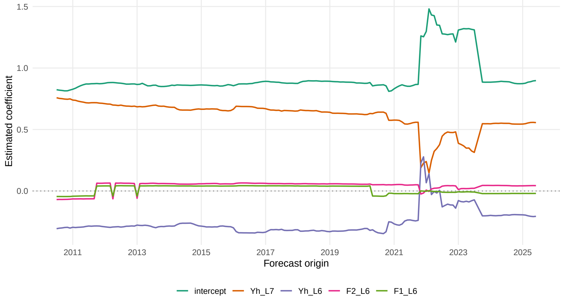
Top-5 most time-varying coefficients of 2SRR-FAVAR (own lags + PCA factor loadings)
