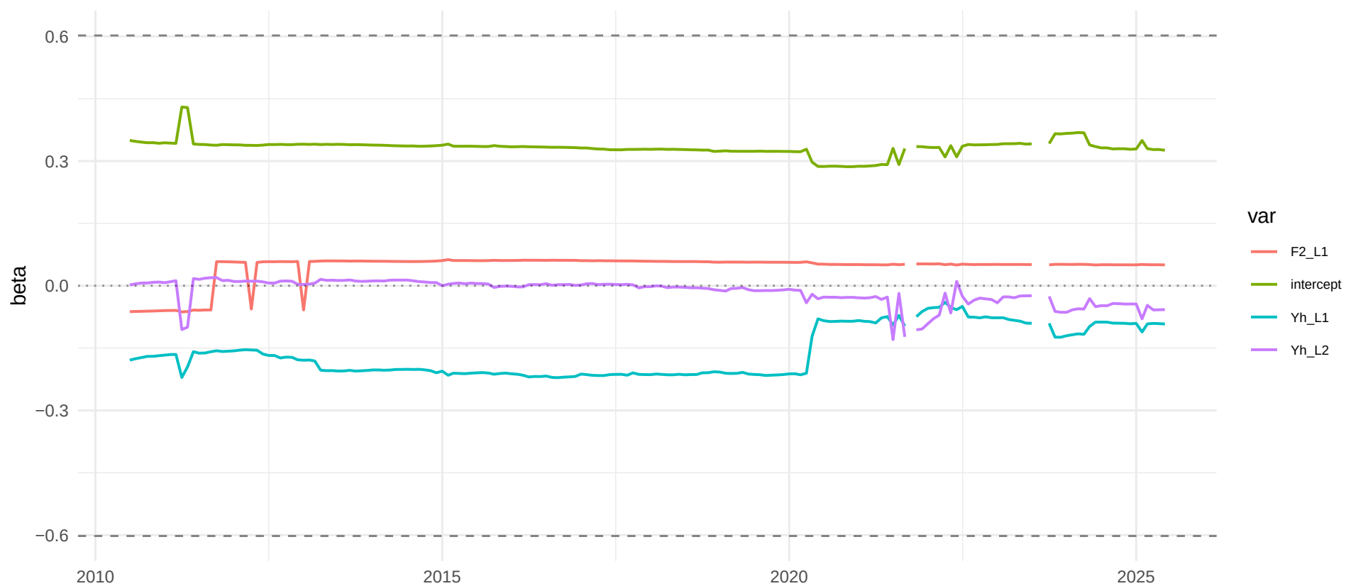
h=1: top-4 TVP (FAVAR) betas vs constant Ridge ( |\text{beta}|=0.602 )
