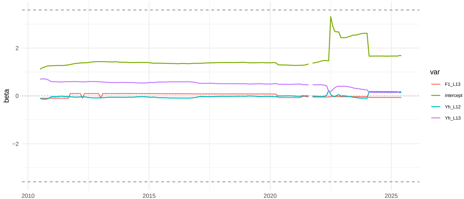
h=12: top-4 TVP (FAVAR) betas vs constant Ridge ( |\text{beta}|=3.591 )
