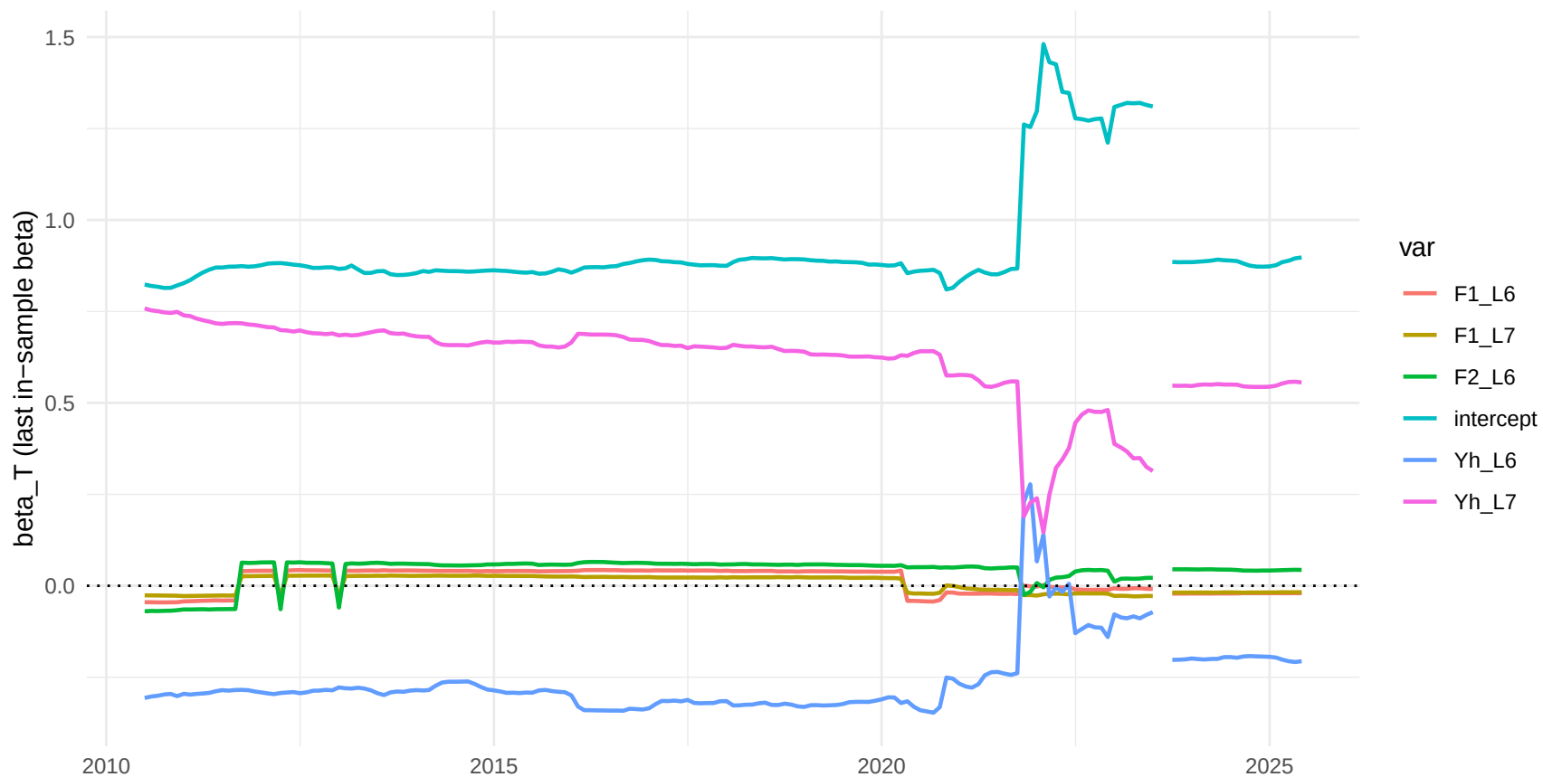
TVP-FAVAR, h=6: top-6 betas (by sd)
