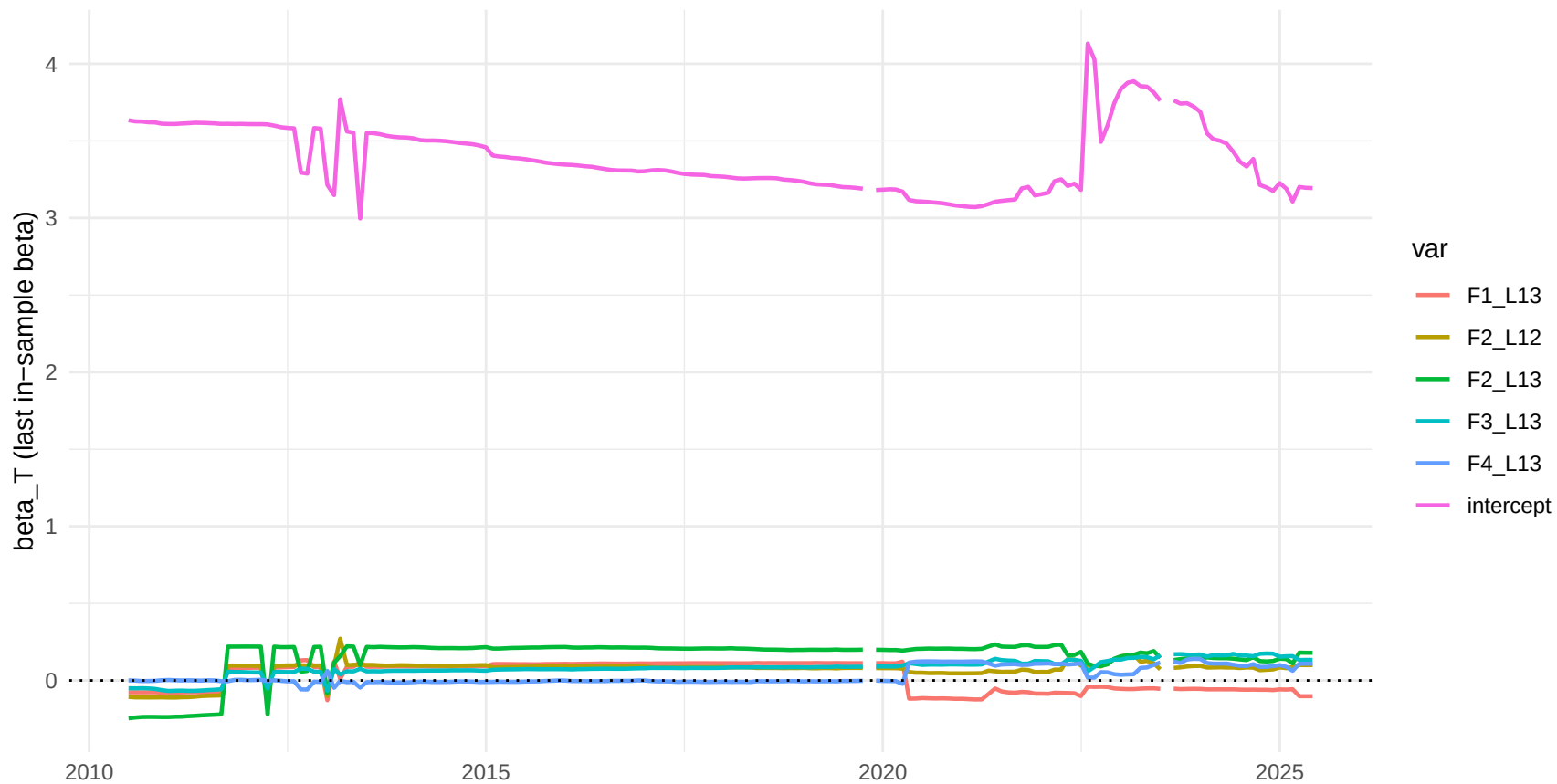
TVP-Factor, h=12: top-6 betas (by sd)
