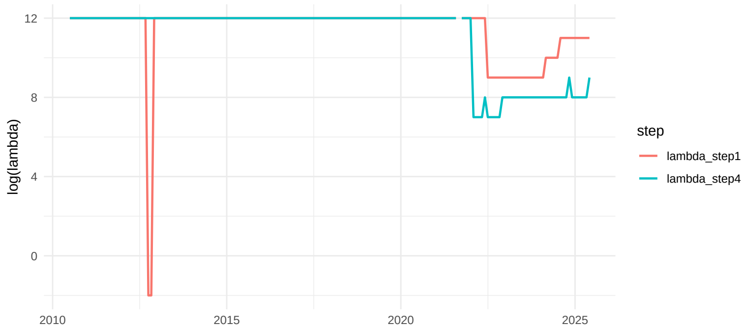
TVP-Factor, h=6: Step1 vs Step4 lambdas (log)
