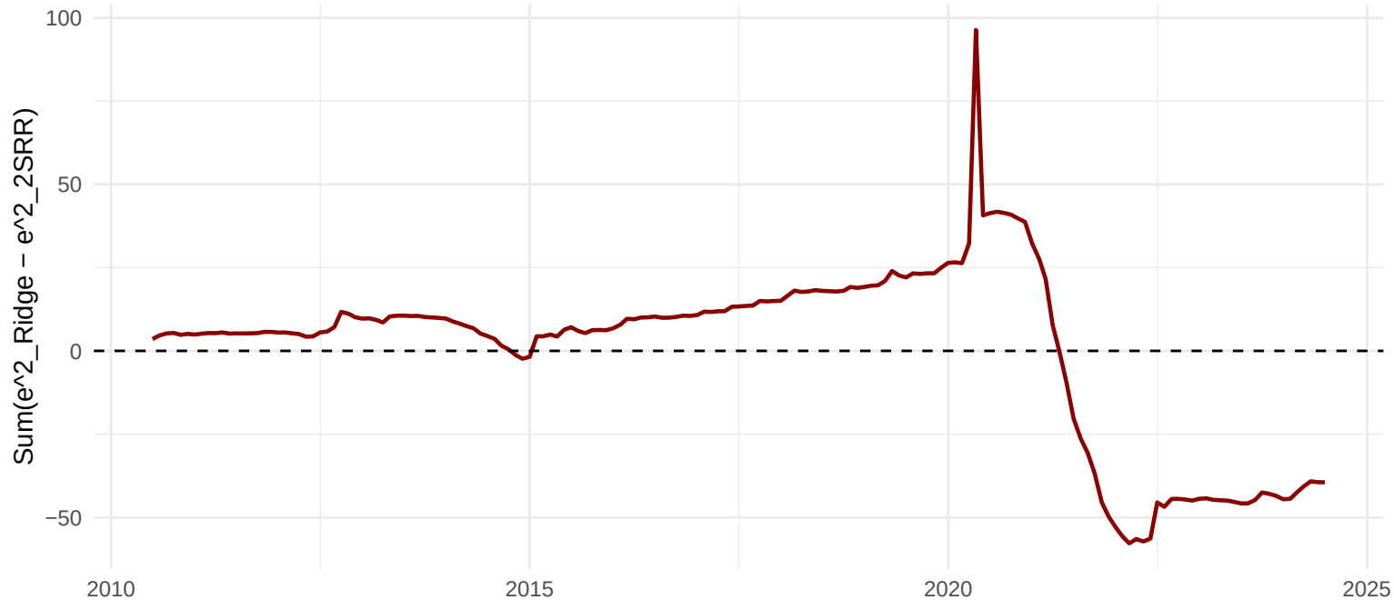
CSSED 2SRR-Factor vs Ridge Step1, h=12
