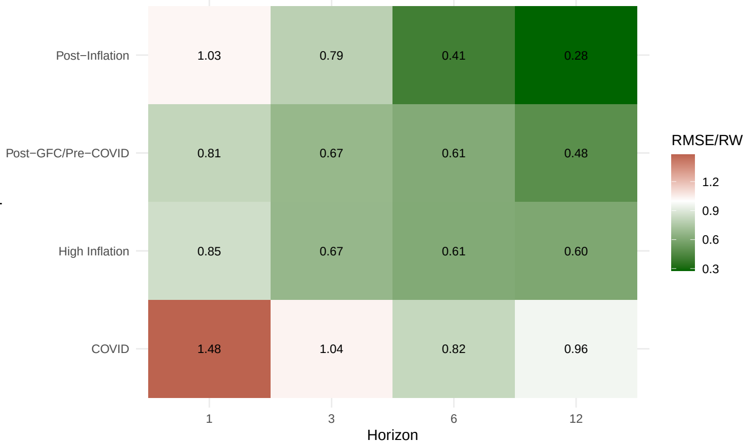
TVP-FAVAR: RMSE relative to RW per sub-period
