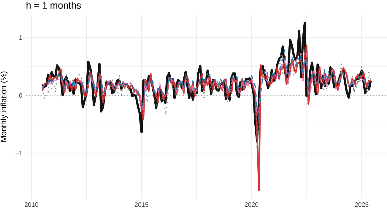
2SRR-FAVAR vs the 3 best Medeiros models — 4 horizons Realized (black) = monthly y_t (identical in all panels). Forecasts h -steps / h = monthly-rate prediction.
