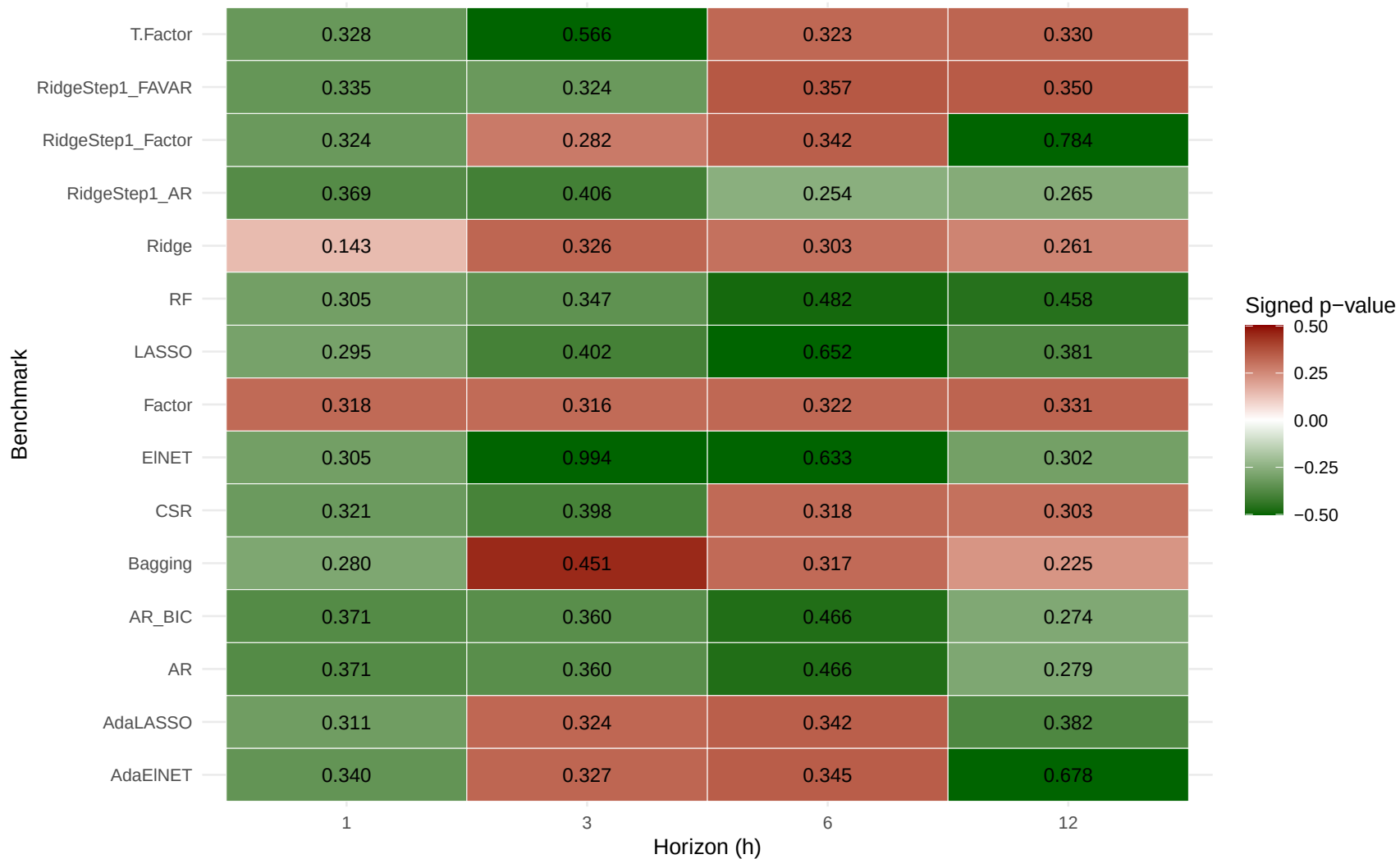
Diebold–Mariano p-values: 2SRR–FAVAR vs each benchmark Green = 2SRR–FAVAR has lower RMSE; Red = benchmark has lower RMSE
