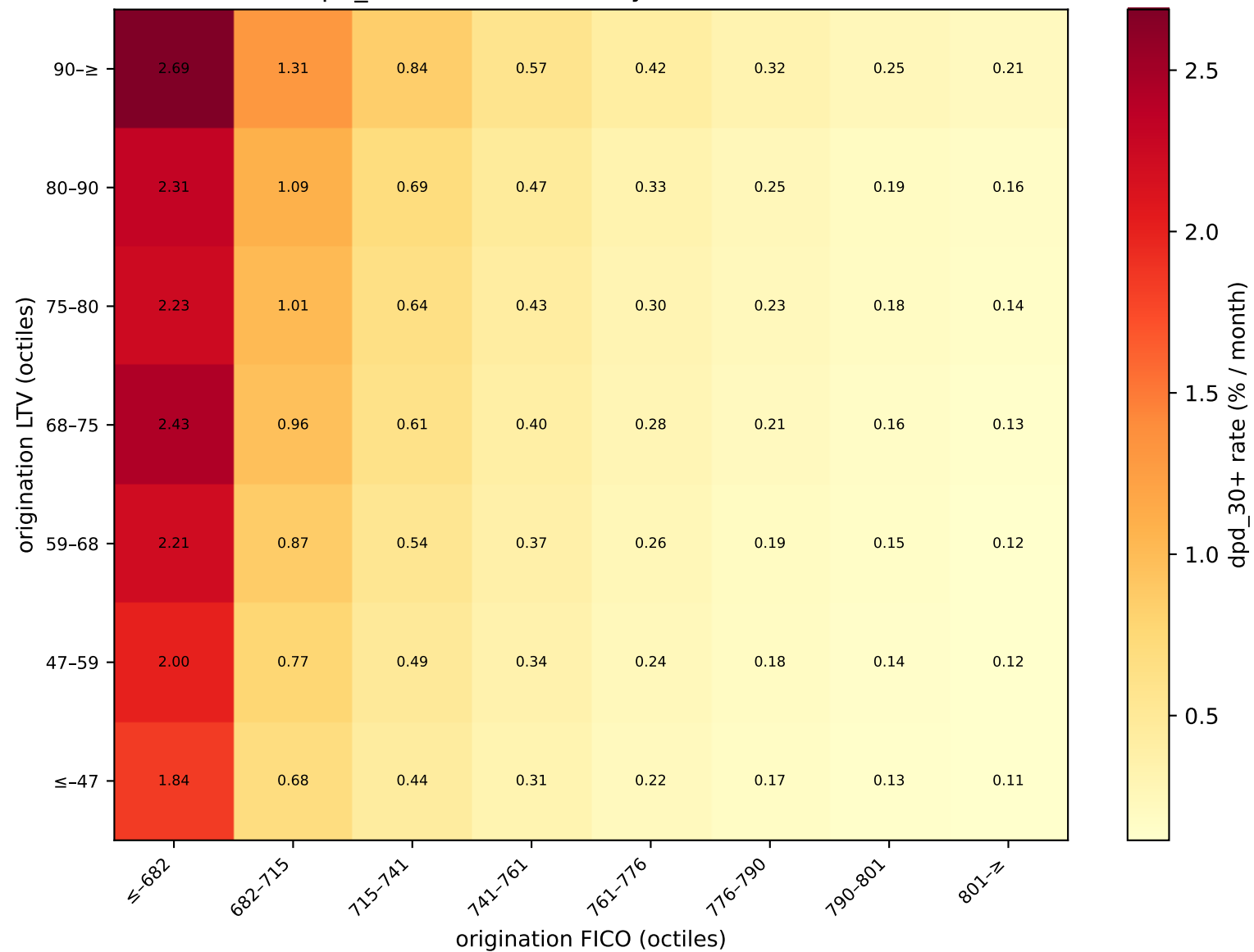
F3.4 current→dpd_30+ rate (% / mo) by FICO × LTV
