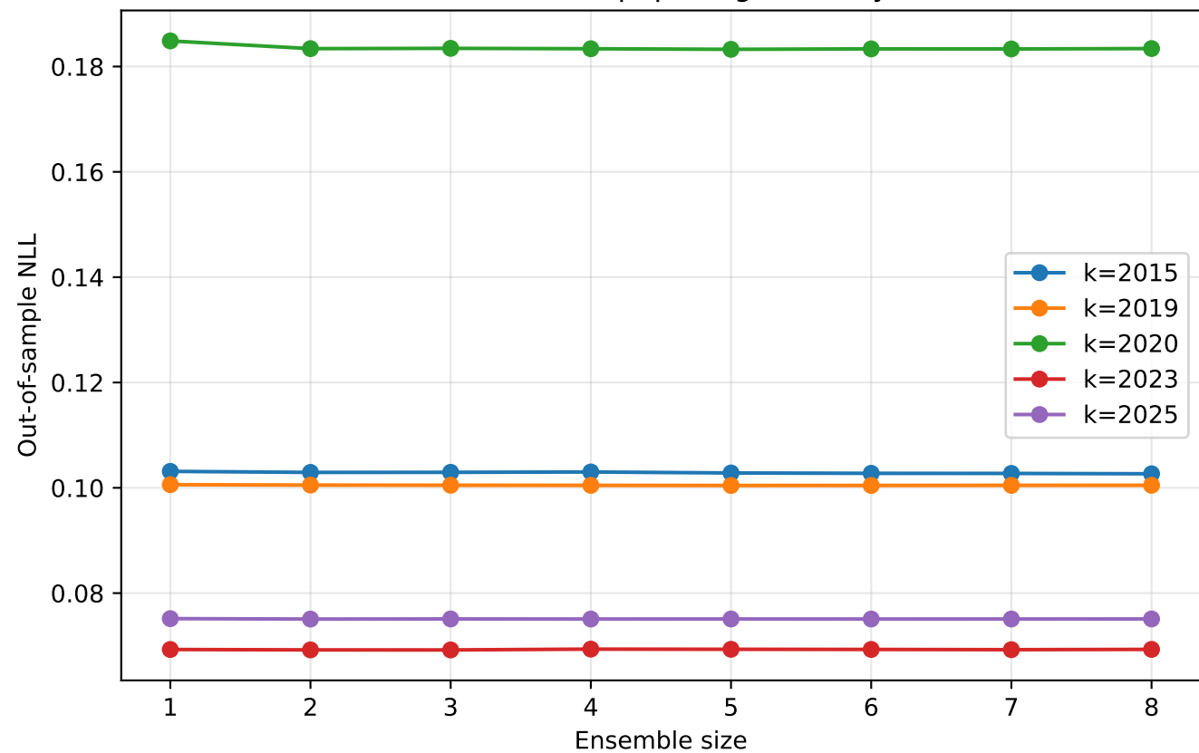
Ensemble-size curve (paper Fig 7) — key windows
