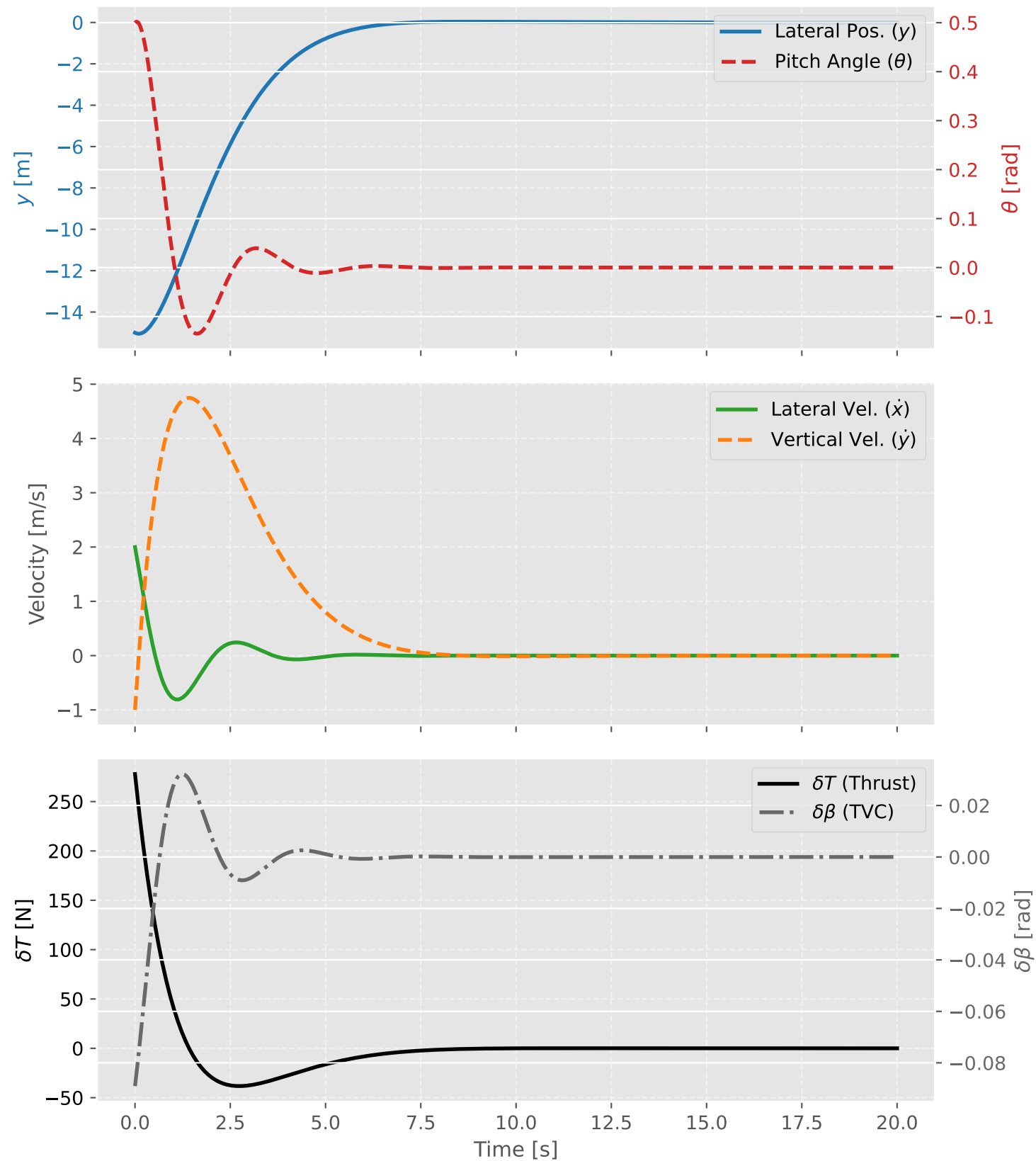
Lander Closed-Loop Response
