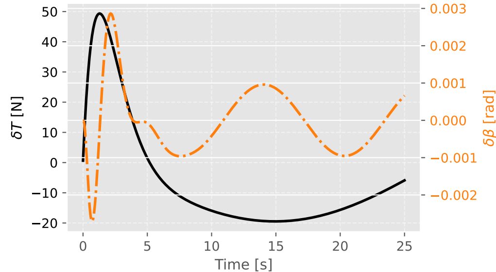
Control Effort &amp; Disturbances
