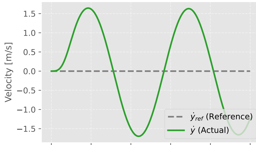
Velocity Tracking
