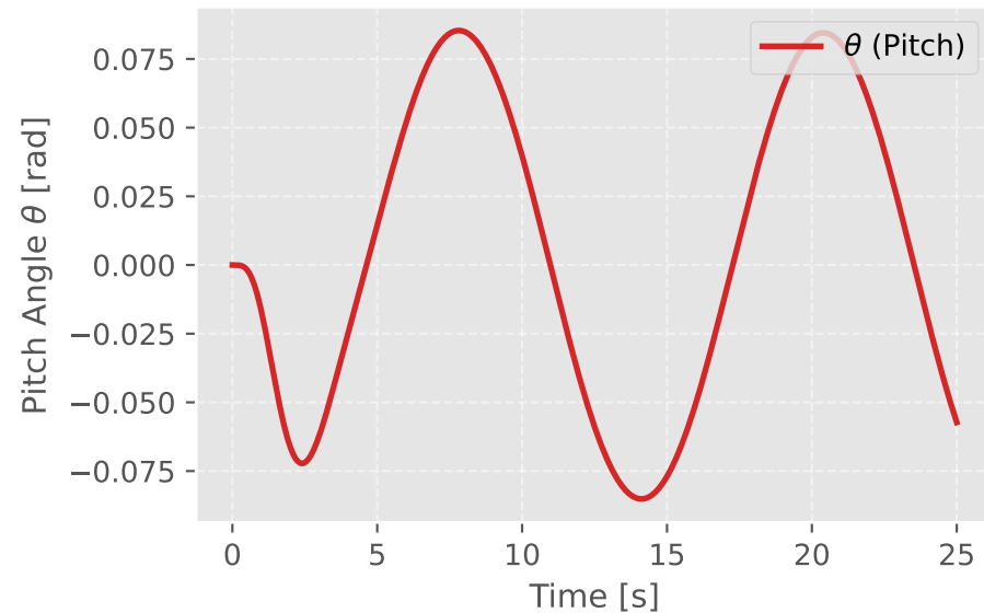
Attitude Dynamics
