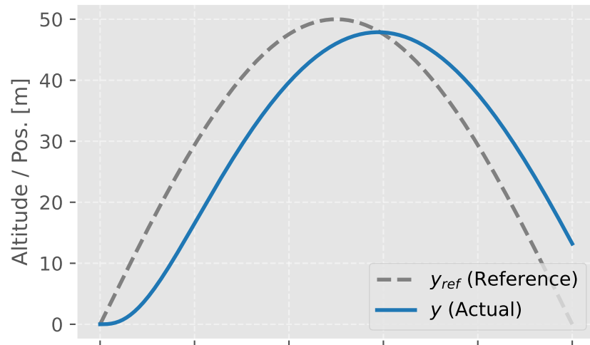
Position Tracking
