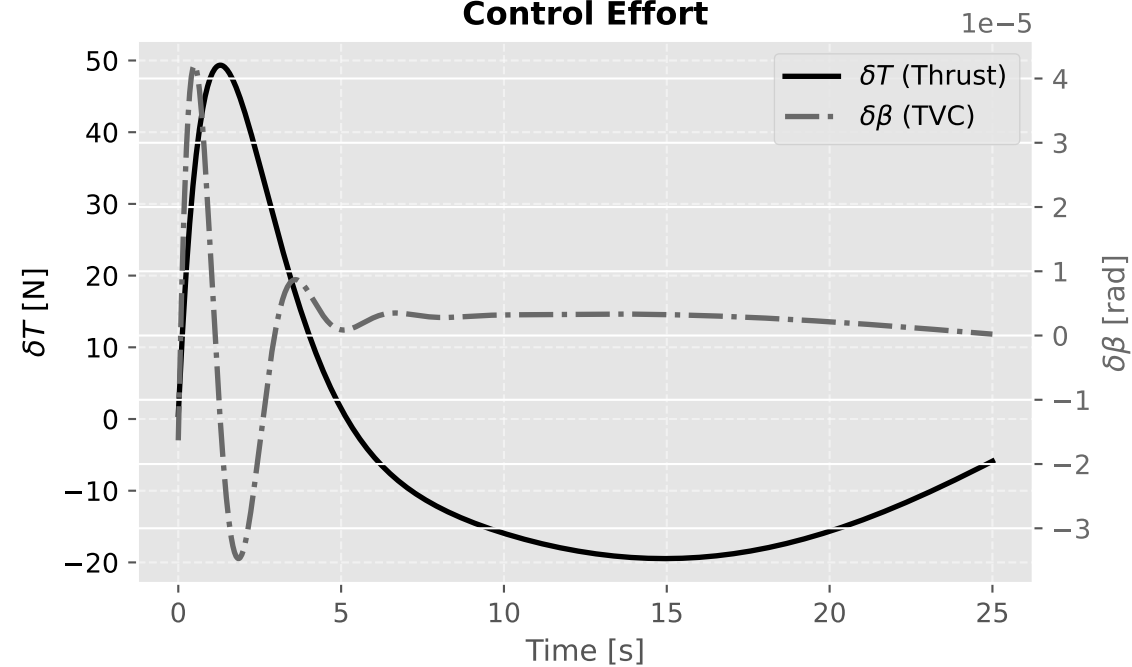
Control Effort
