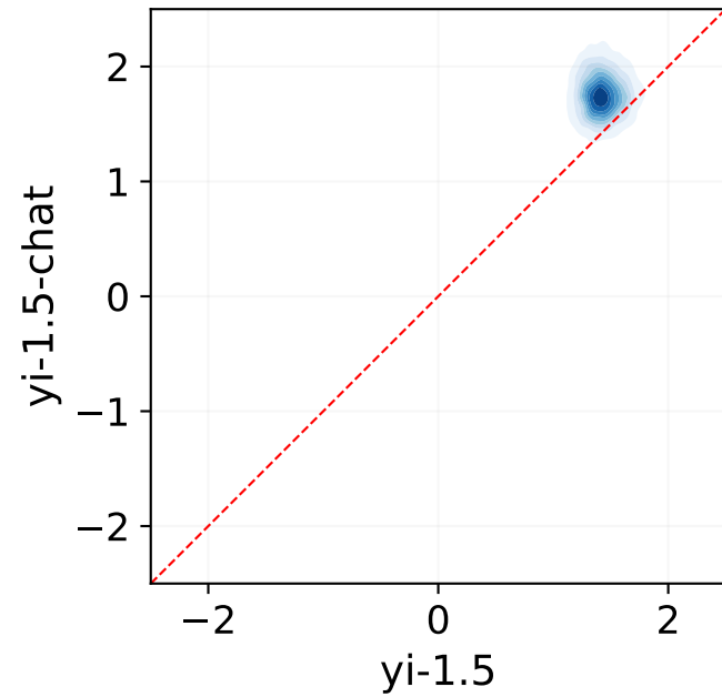
Factor \alpha_1 : MATH
