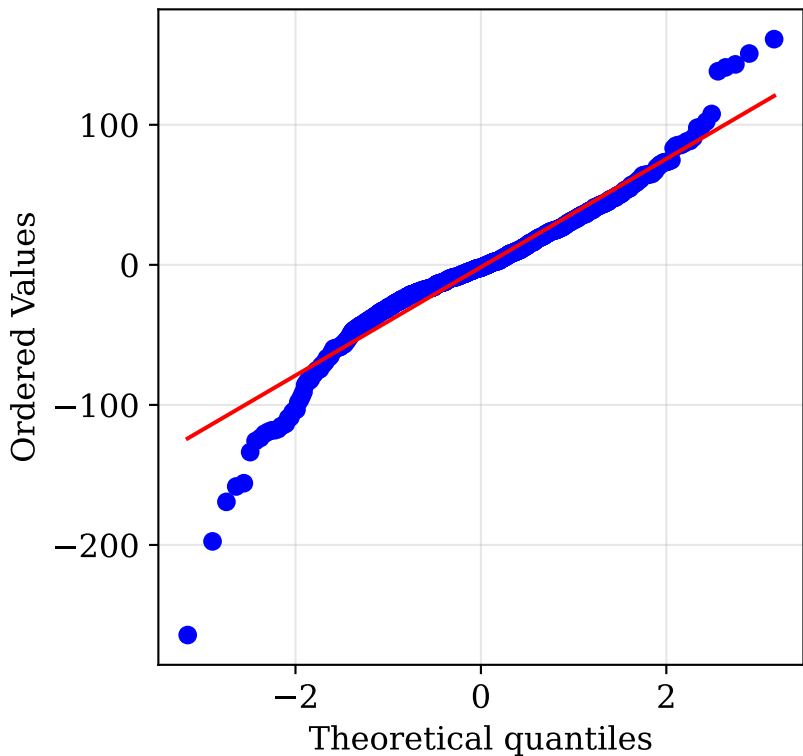
QQ-Plot - BiLSTM
